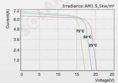
SLP100-12 I-V Curves
