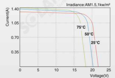
SLP020-12 I-V Curves
